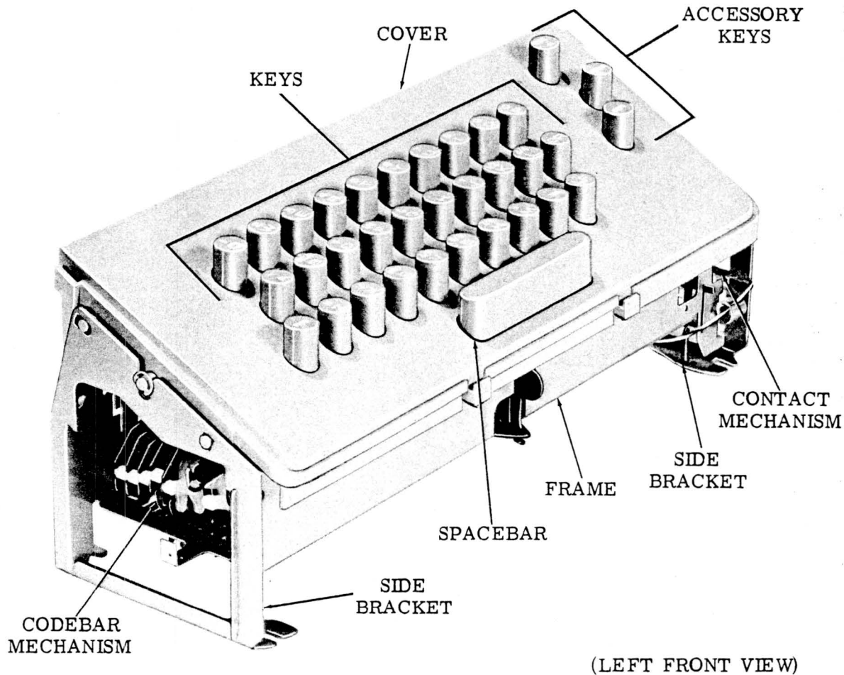
Figure 6 - 32 Keyboard
