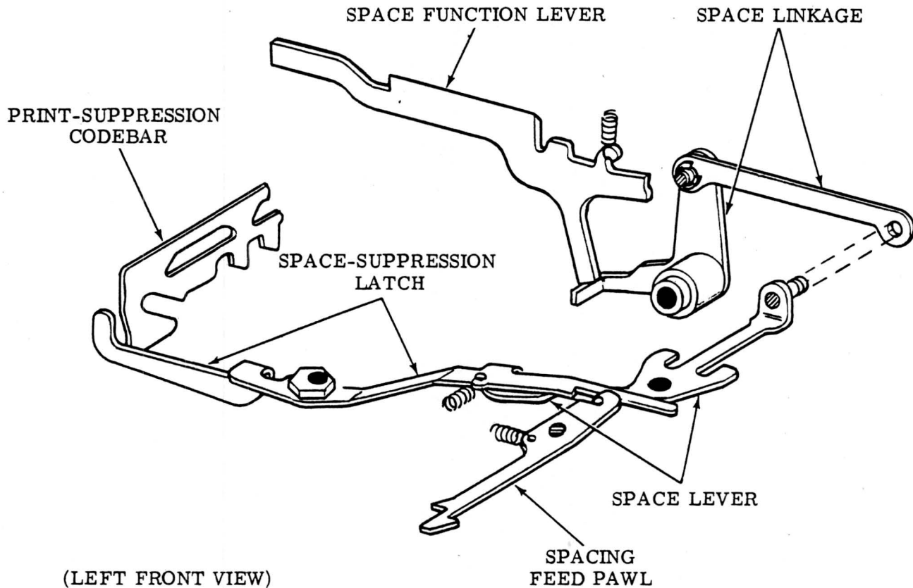
Figure 24 — Space Function and Space-Suppression Mechanism
