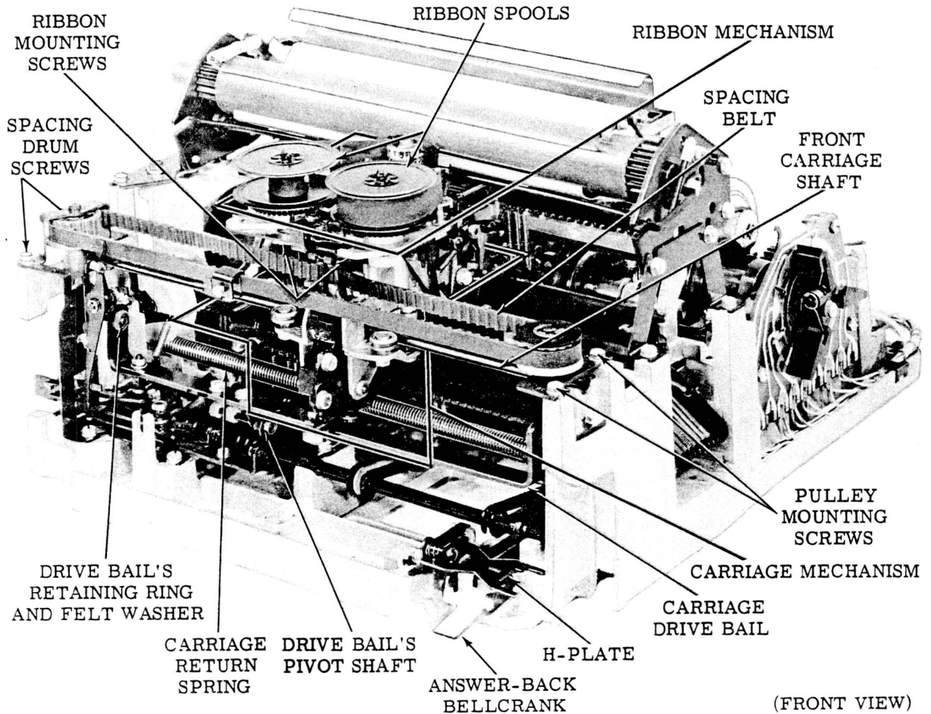
Figure 2 — Typing Unit
