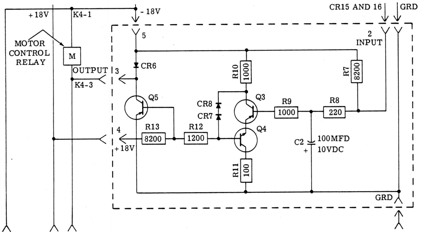
Figure 9 - Motor Delay Timer Circuit
