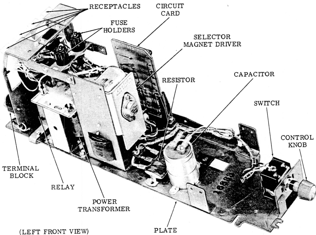
Figure 12 — Typical Call Control Unit
