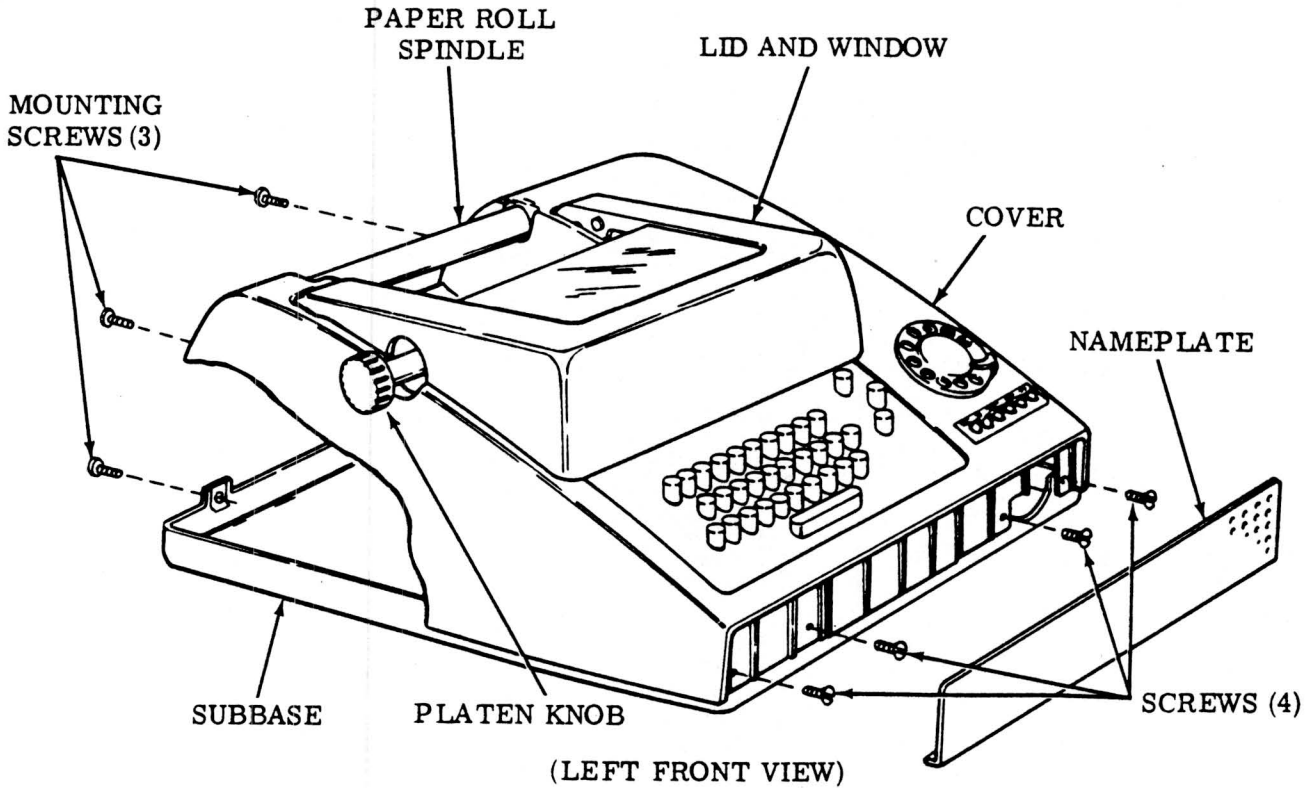
Figure 1 - Cover Mounting
