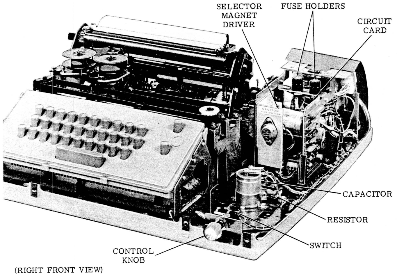
Figure 13 — Keyboard Send-Receive (KSR) Teletypewriter Set with Call Control Unit
