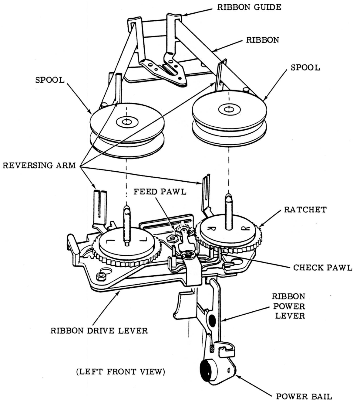
Figure 22 - Ribbon Mechanism
