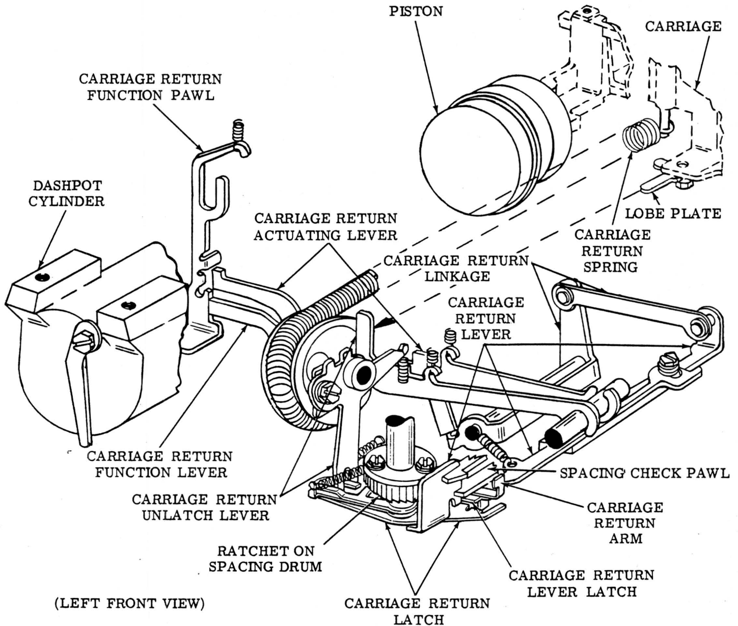
Figure 25 — Carriage Return Mechanism
