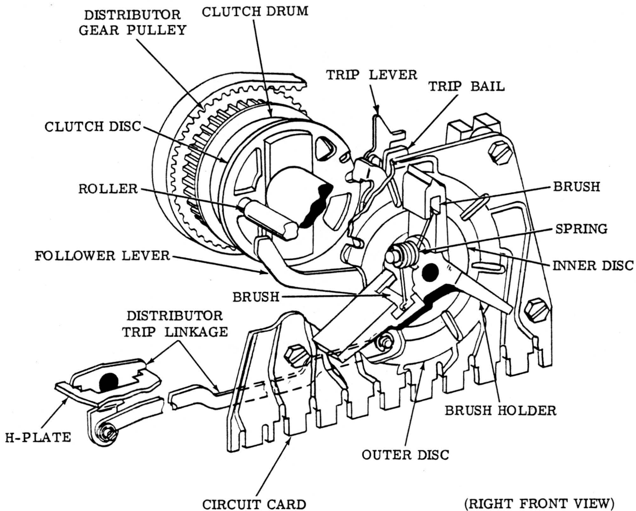
Figure 8 - Distributor Mechanism
