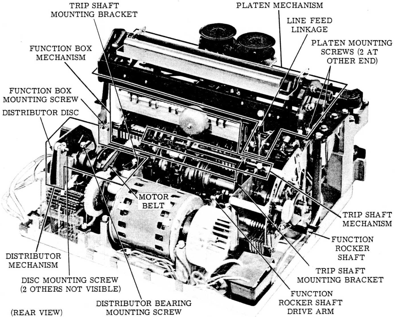
Figure 3 — Typing Unit
