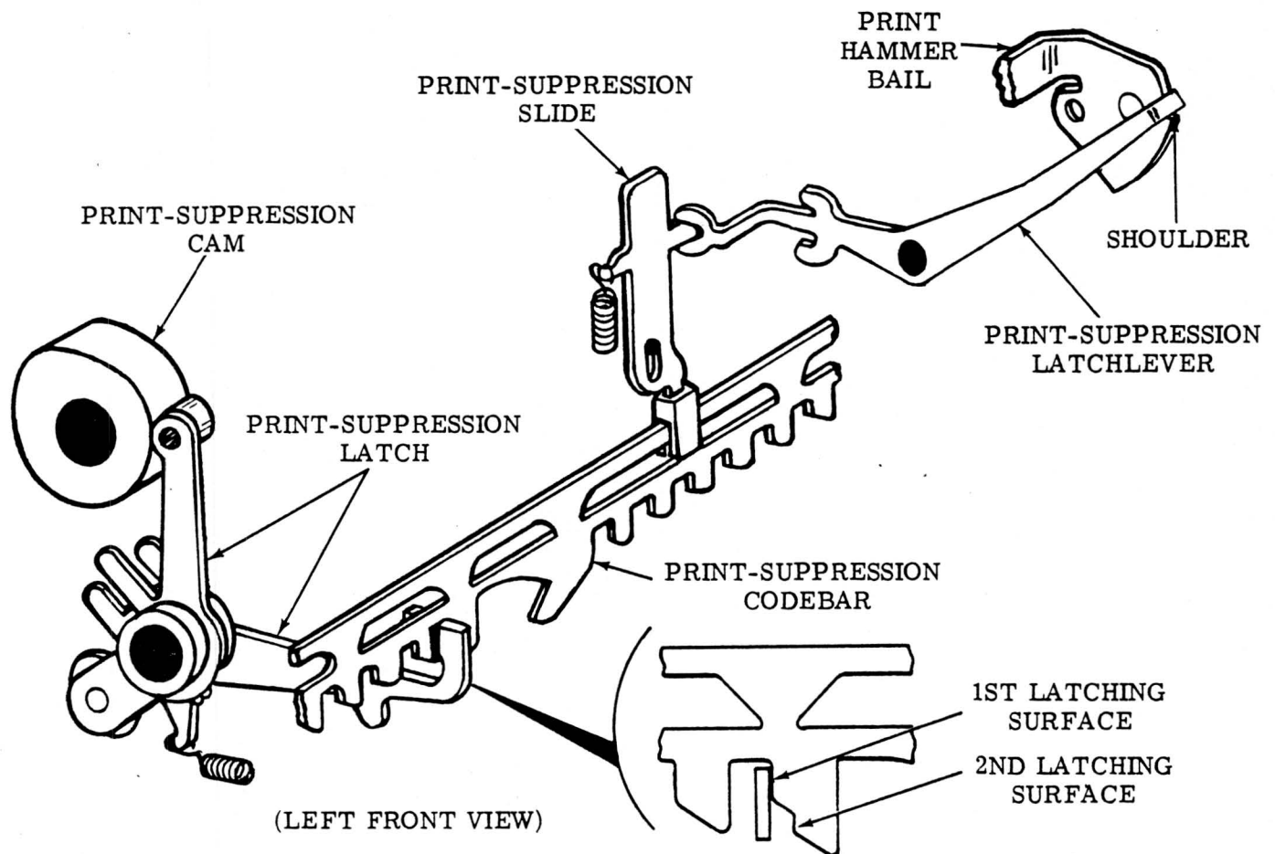
Figure 21 — Print Suppression Mechanism
