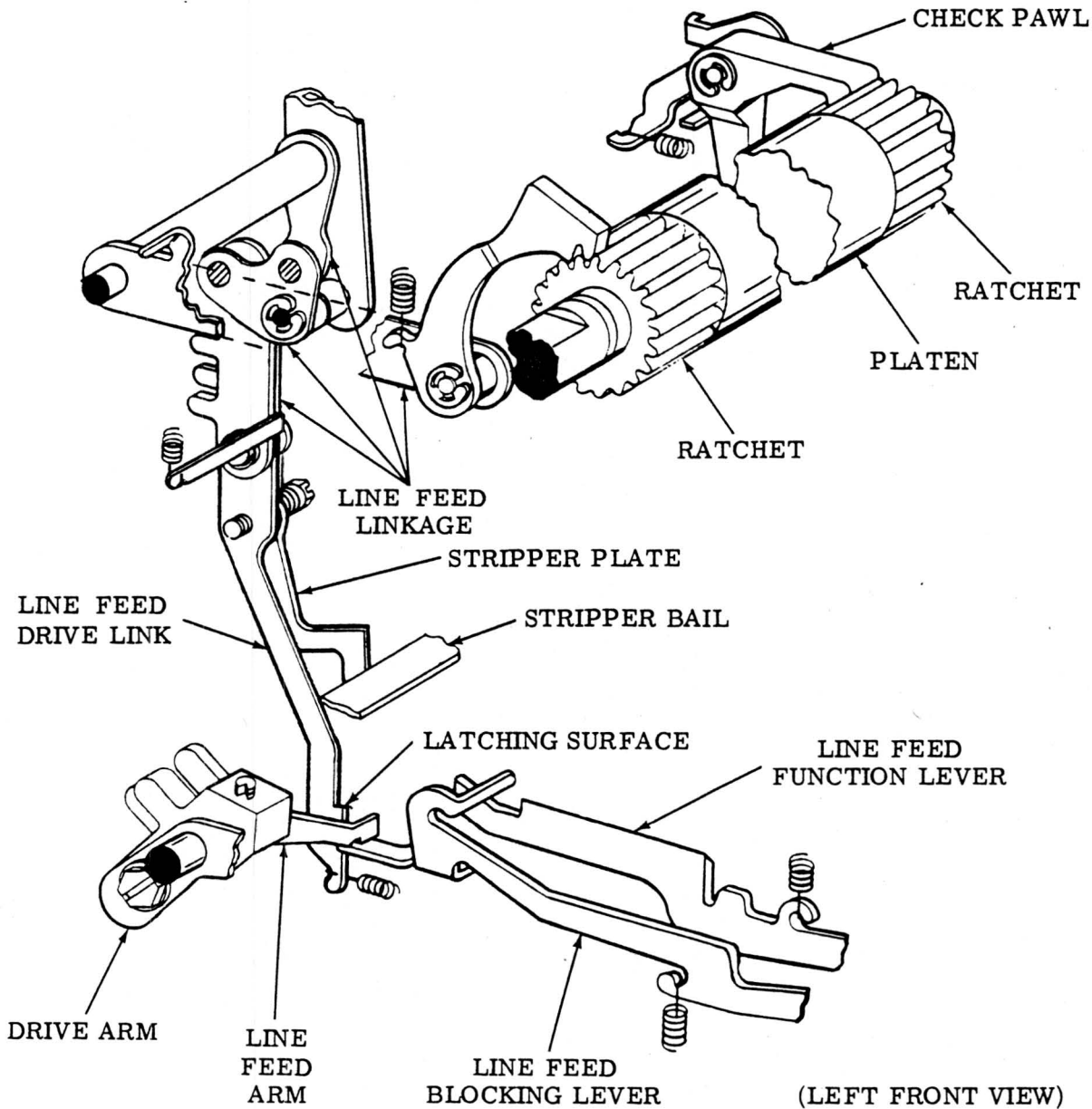
Figure 26 — Paper Feed Mechanism (Friction Feed).
