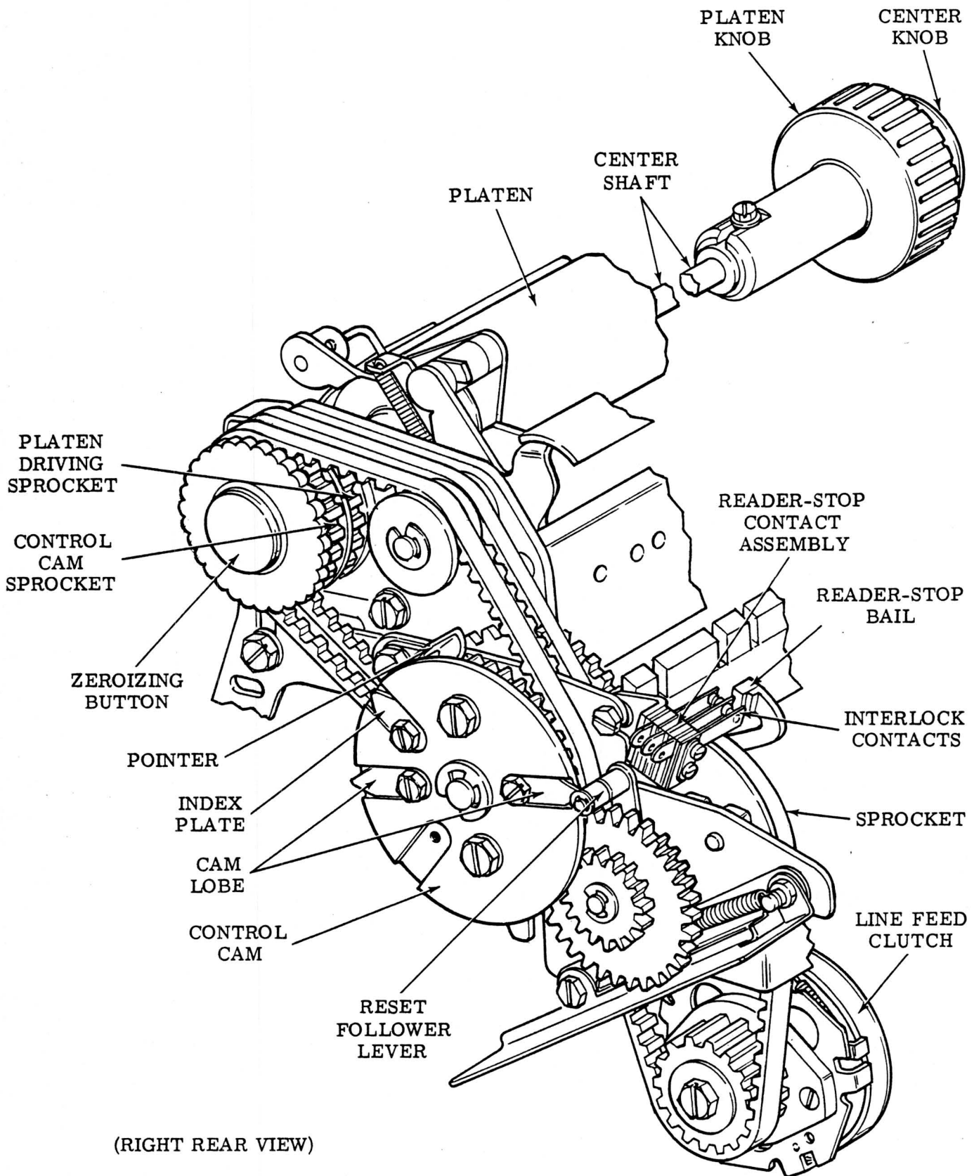
Figure 27 — Platen Drive Mechanism (Sprocket Feed)
