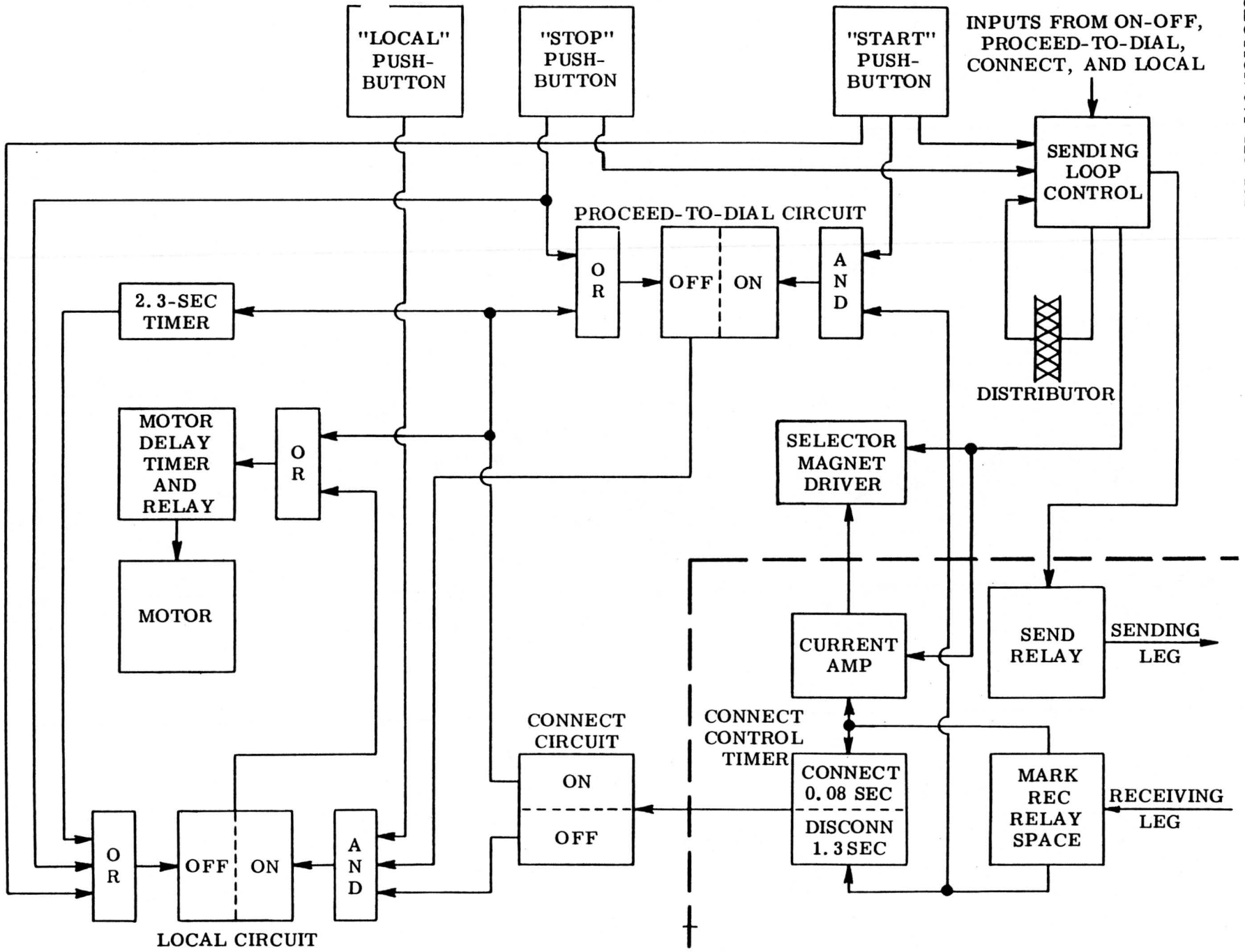
Figure 10 - Block Diagram—Polar Adapter Circuit
