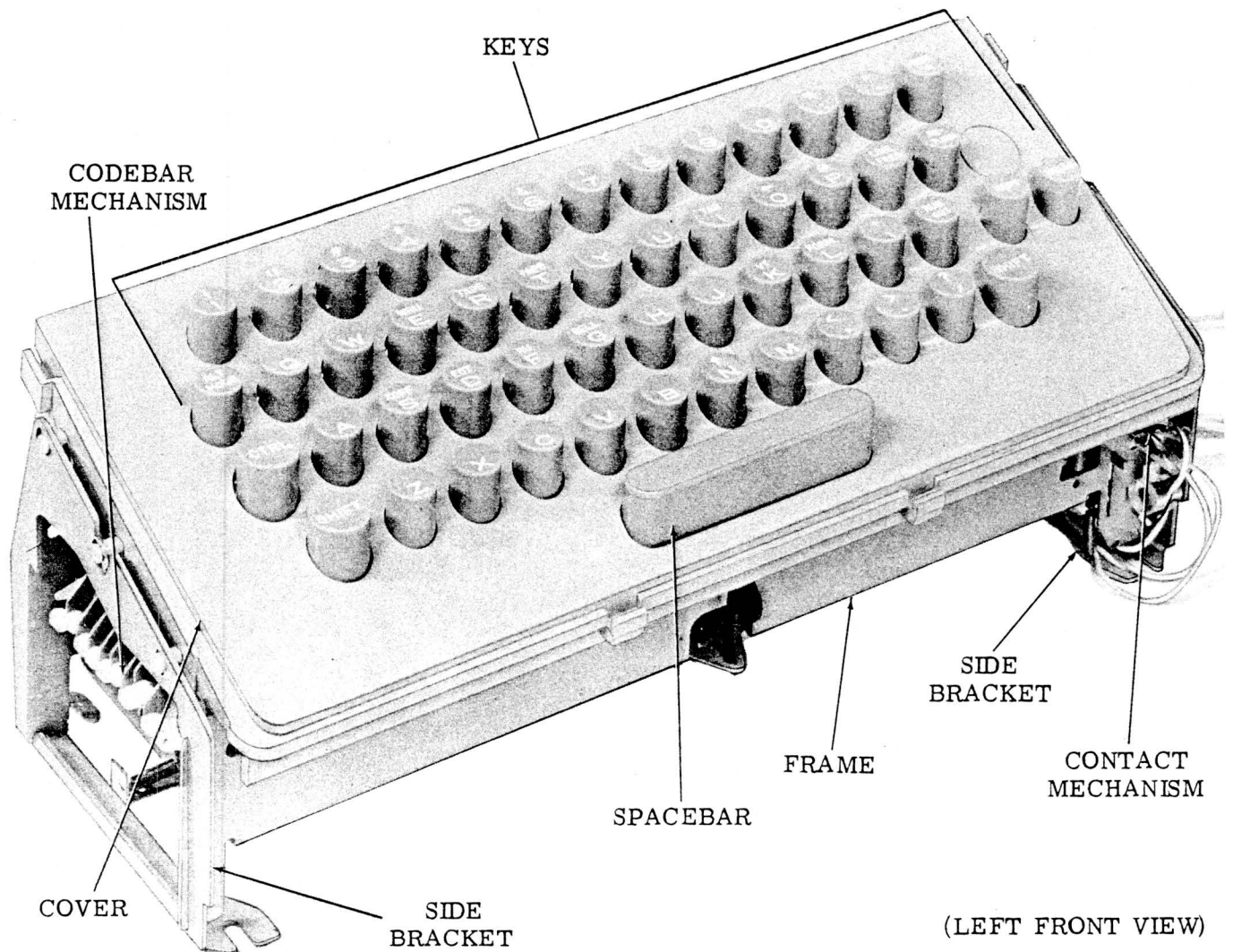
Figure 7 - 33 Keyboard
