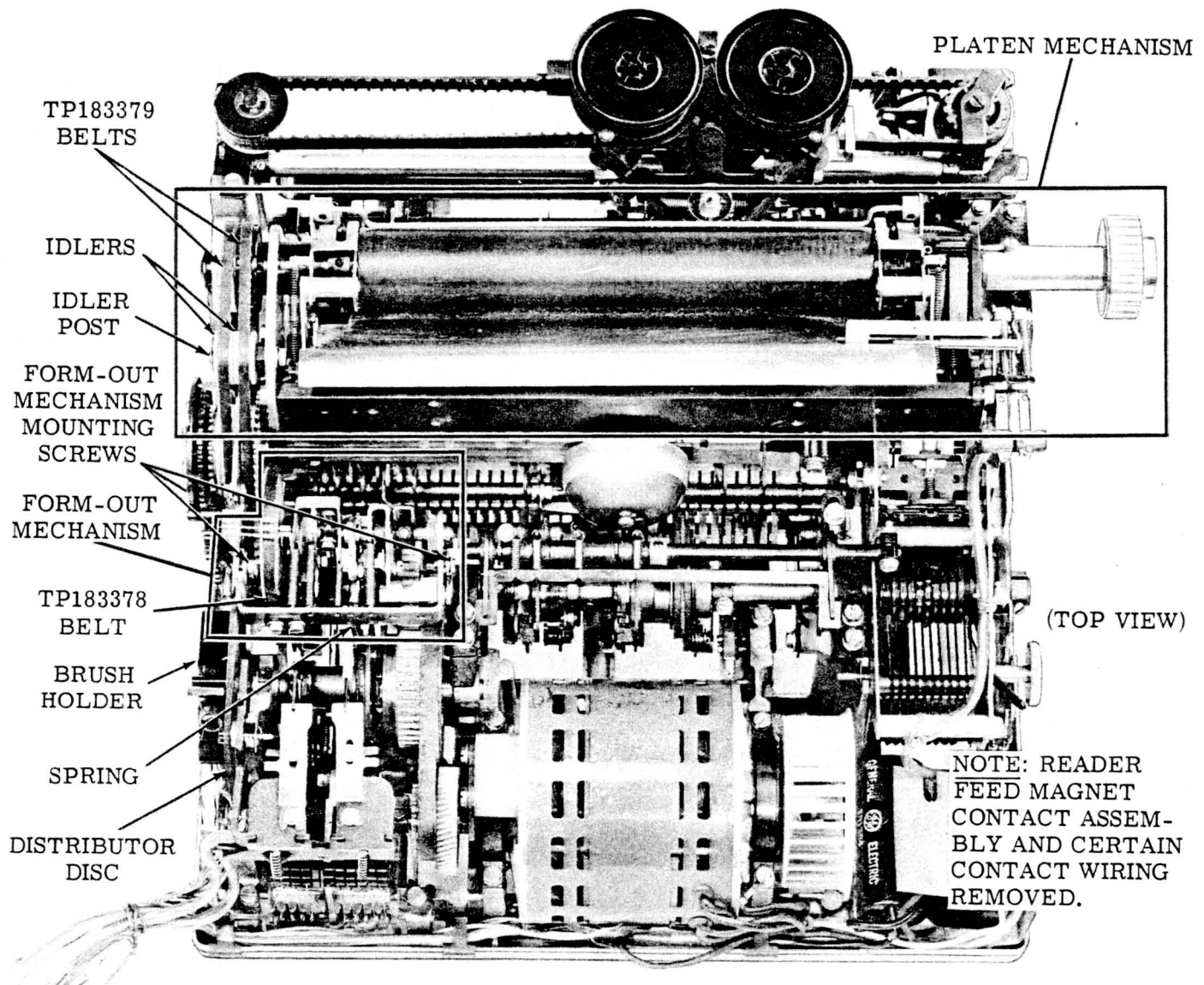
Figure 8 - Typing Unit
