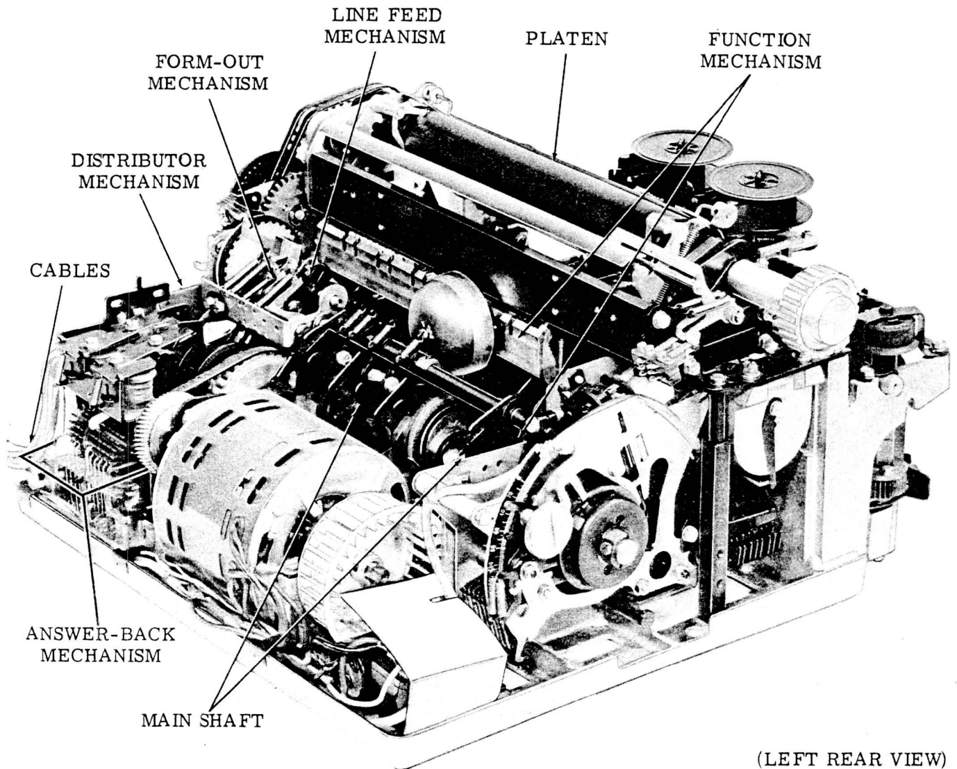
Figure 9 — Typing Unit (Sprocket Feed)
