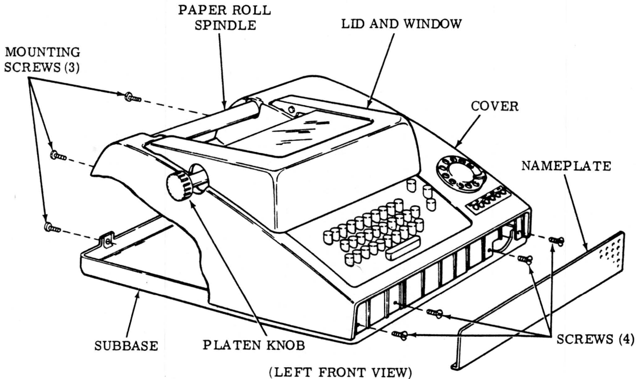
Figure 2 - Cover
