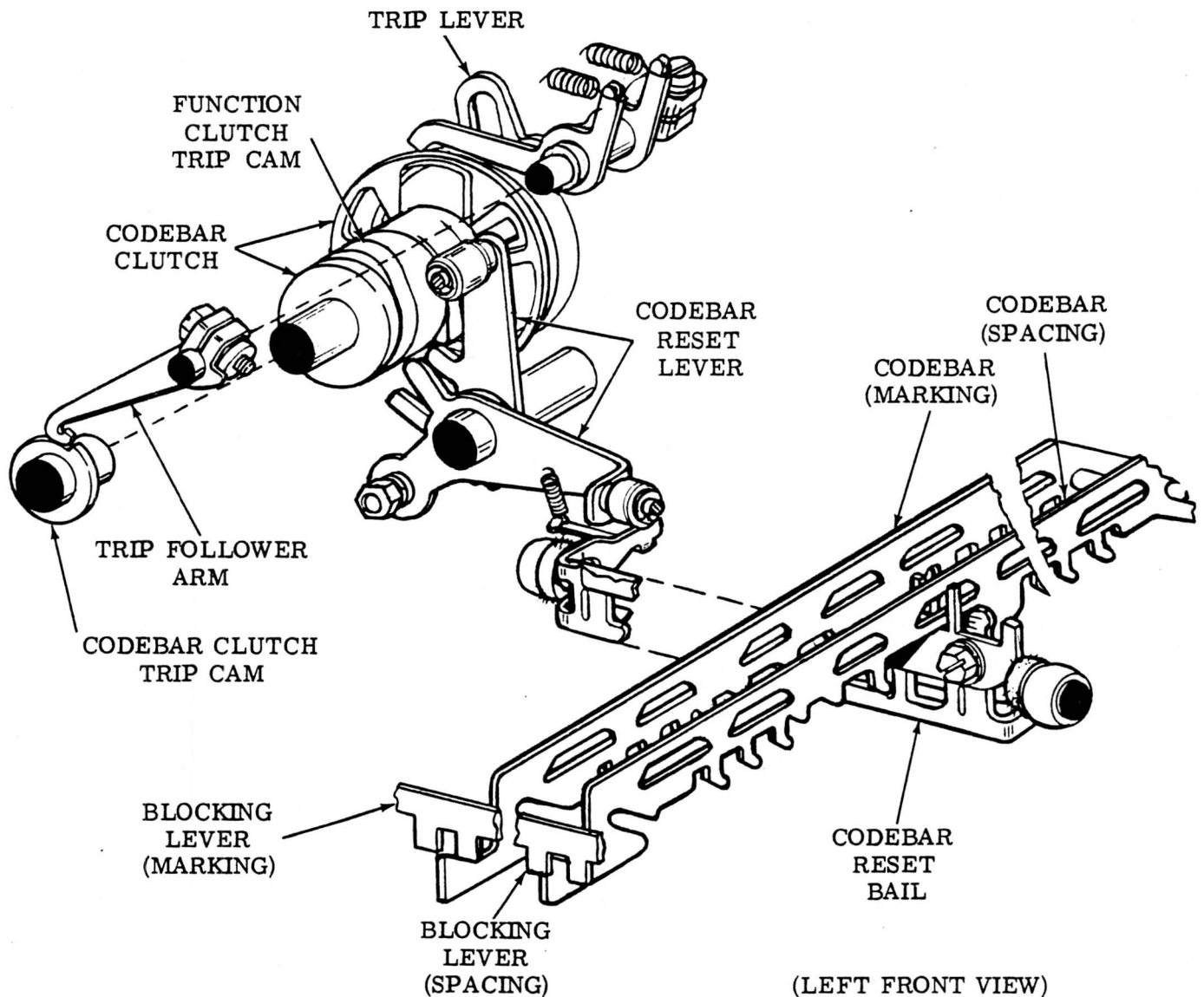
Figure 12 - Codebar Mechanism
