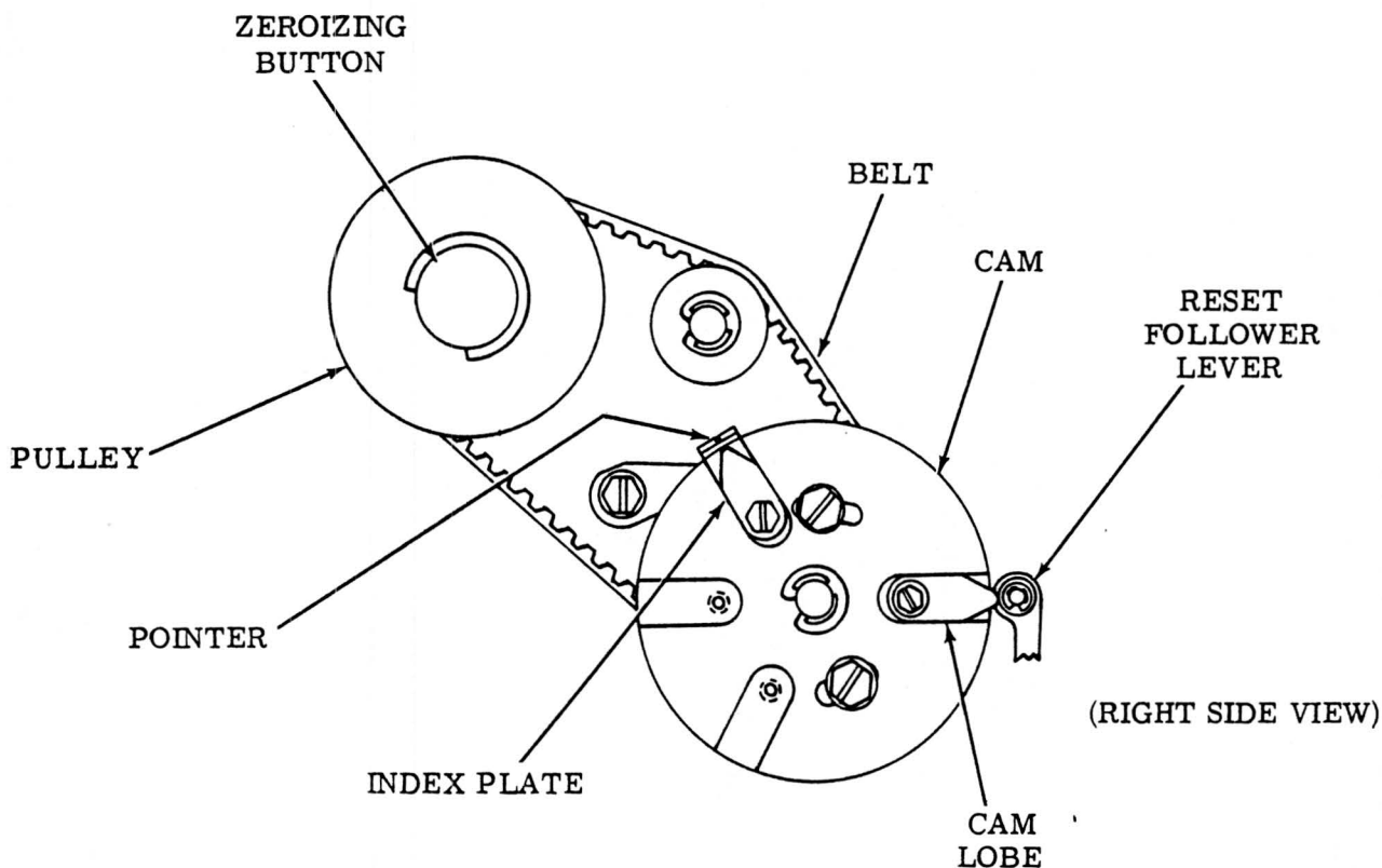
Figure 8 - Zeroizing Position of Platen Drive Mechanism — One Cam Lobe Operation
