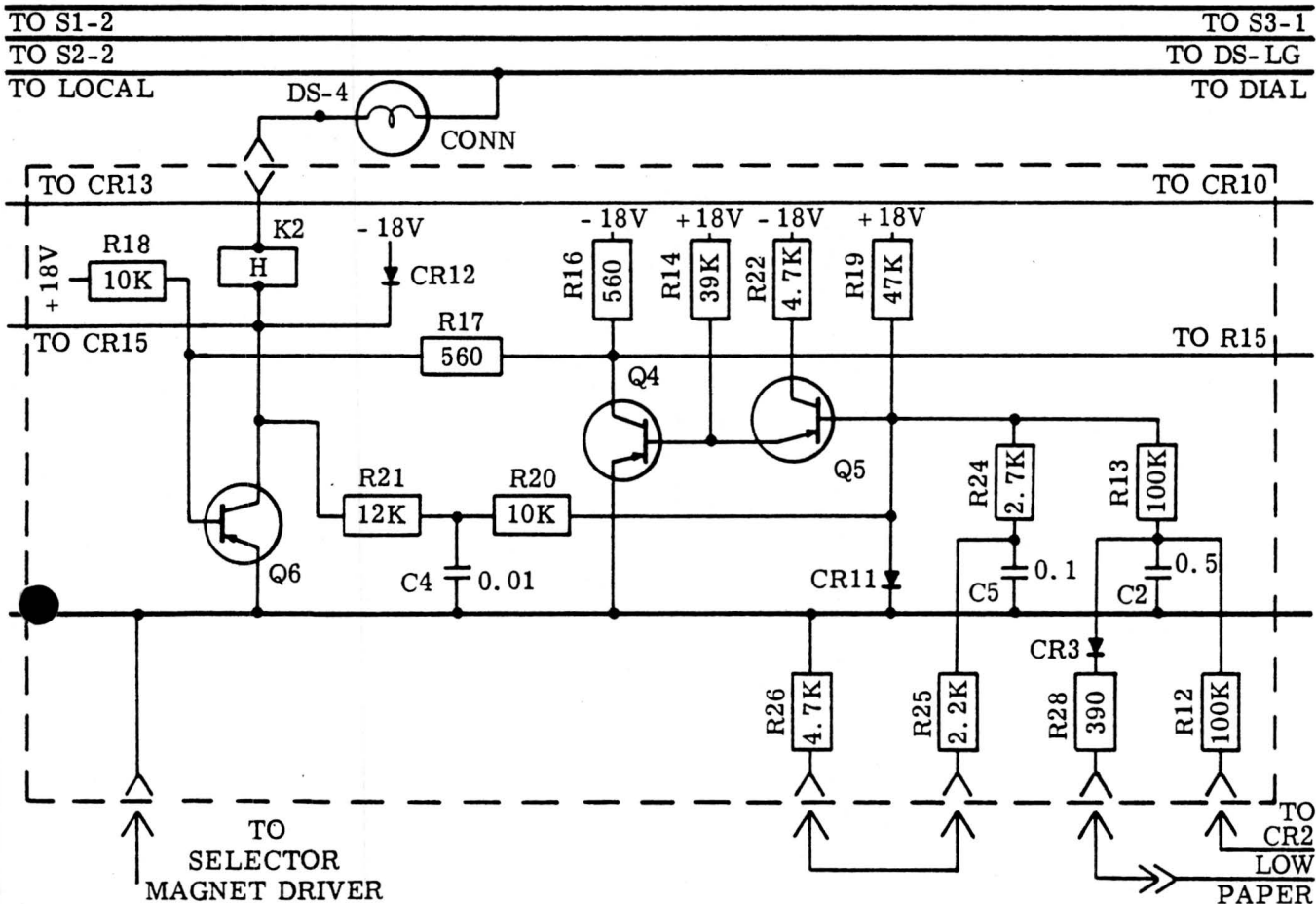
Figure 3 - Connect Circuit
