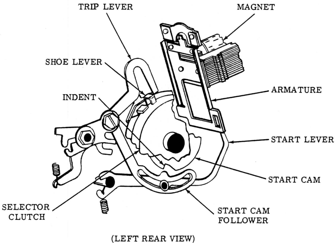
Figure 10 - Selector Trip Mechanism
