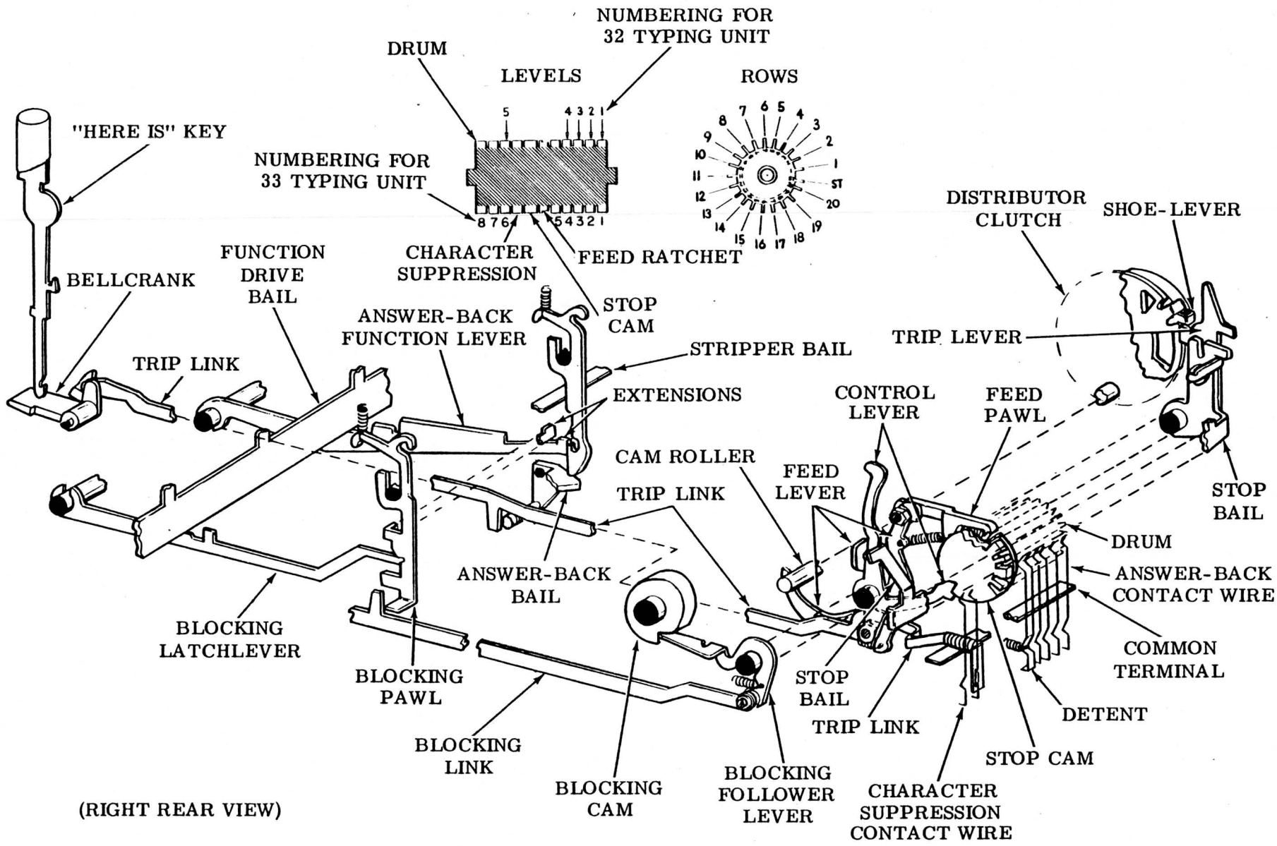
Figure 30 - Answer-Back Mechanism
