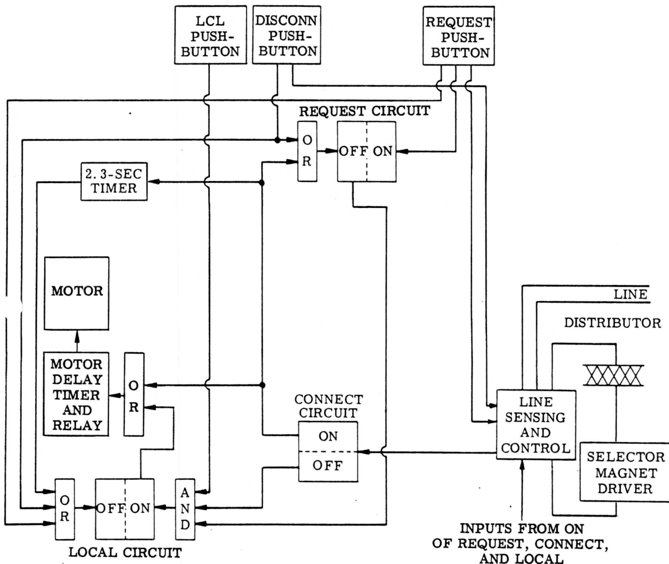
Figure 18 - Block Diagram of Control Circuits
