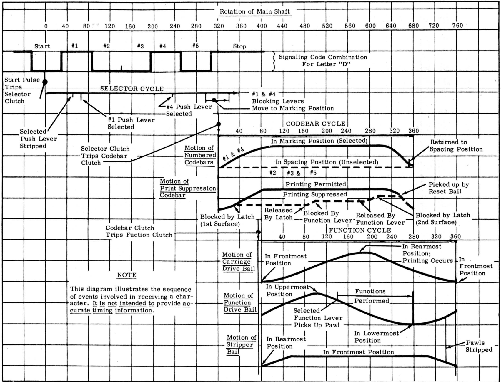
Figure 4 - Sequence Diagram - 32 Typing Unit Operation
