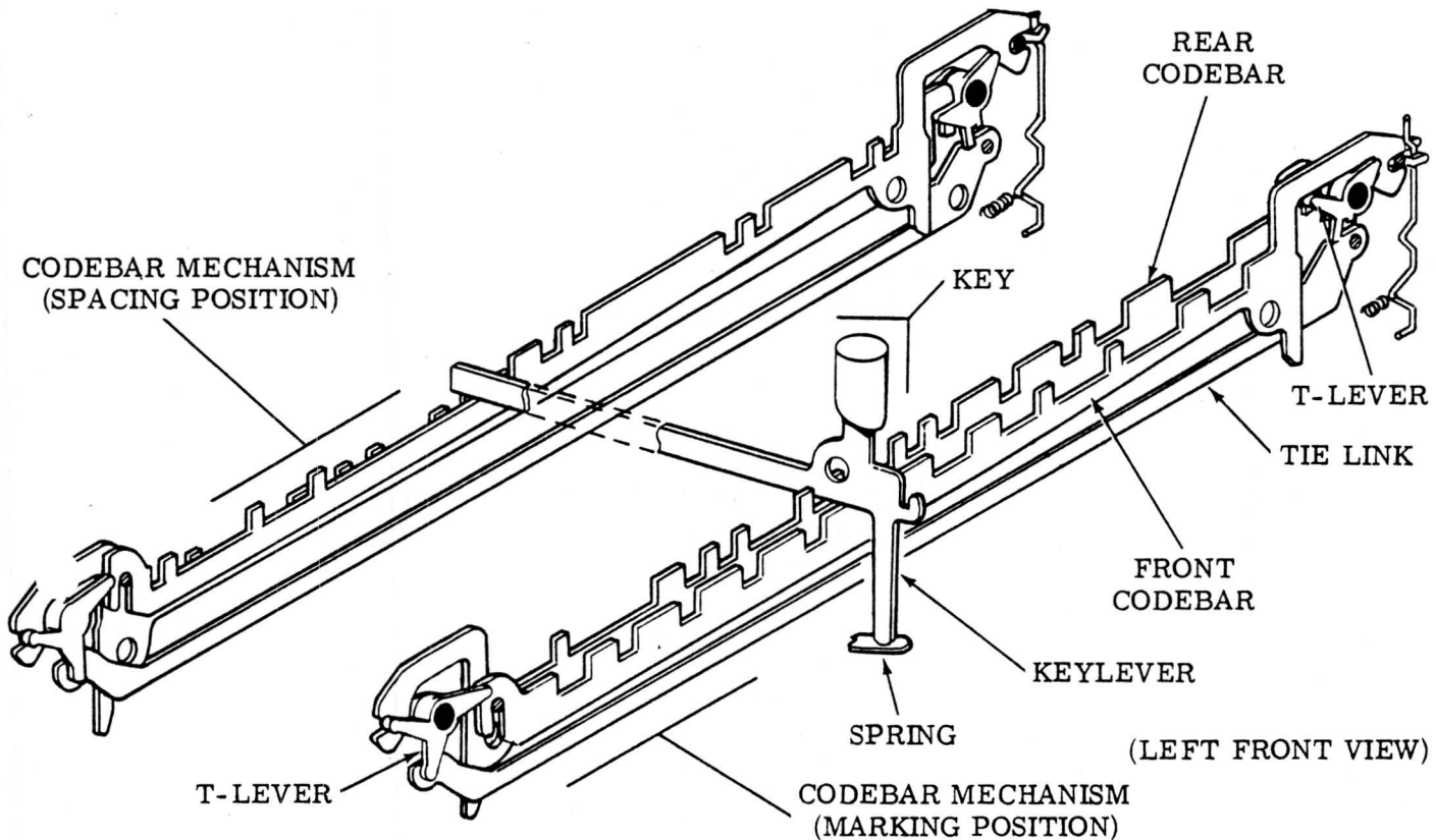
Figure 1 - Codebar Mechanism
