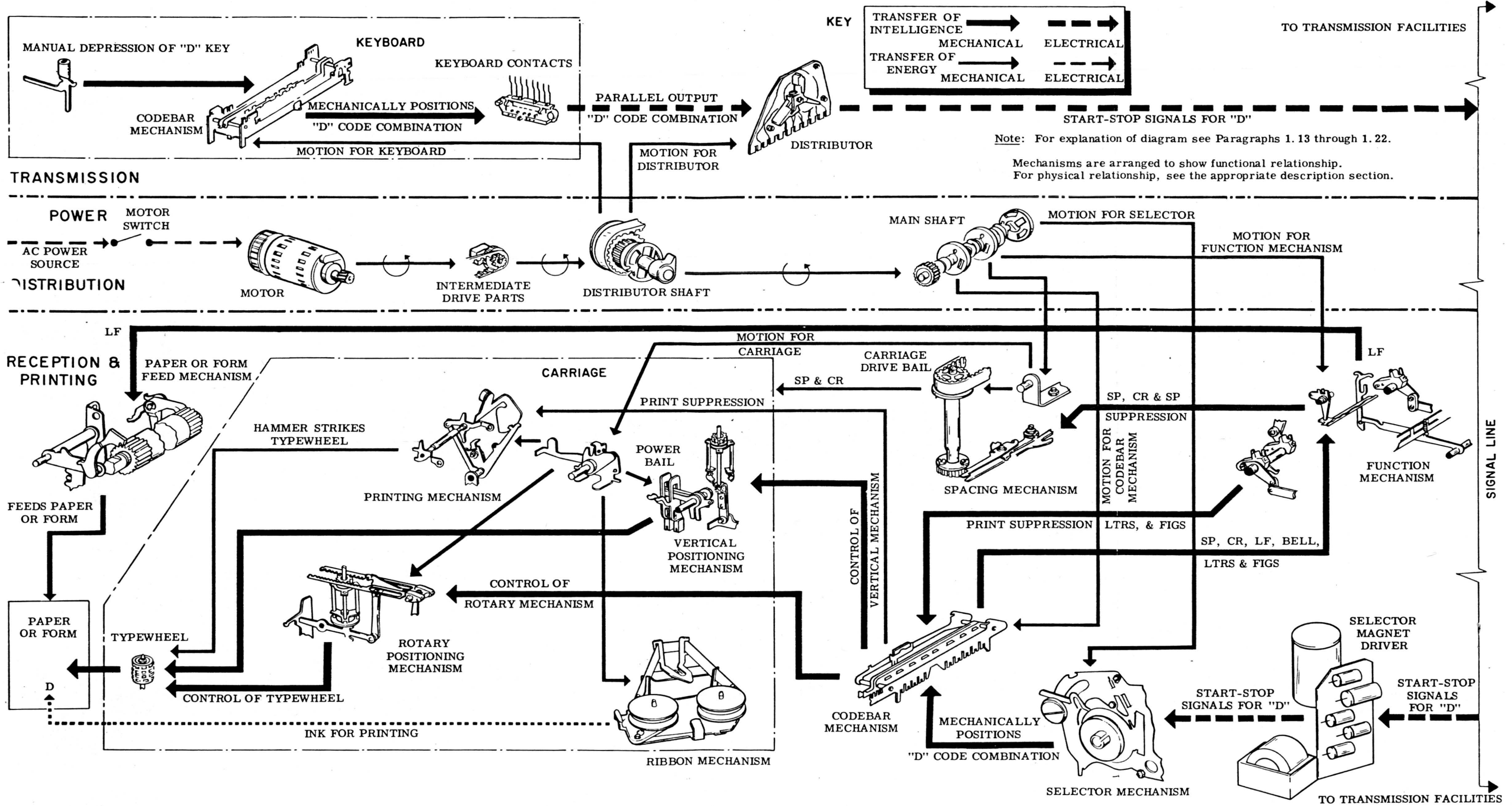
Figure 3 - Schematic Diagram - Typing Unit Operation
