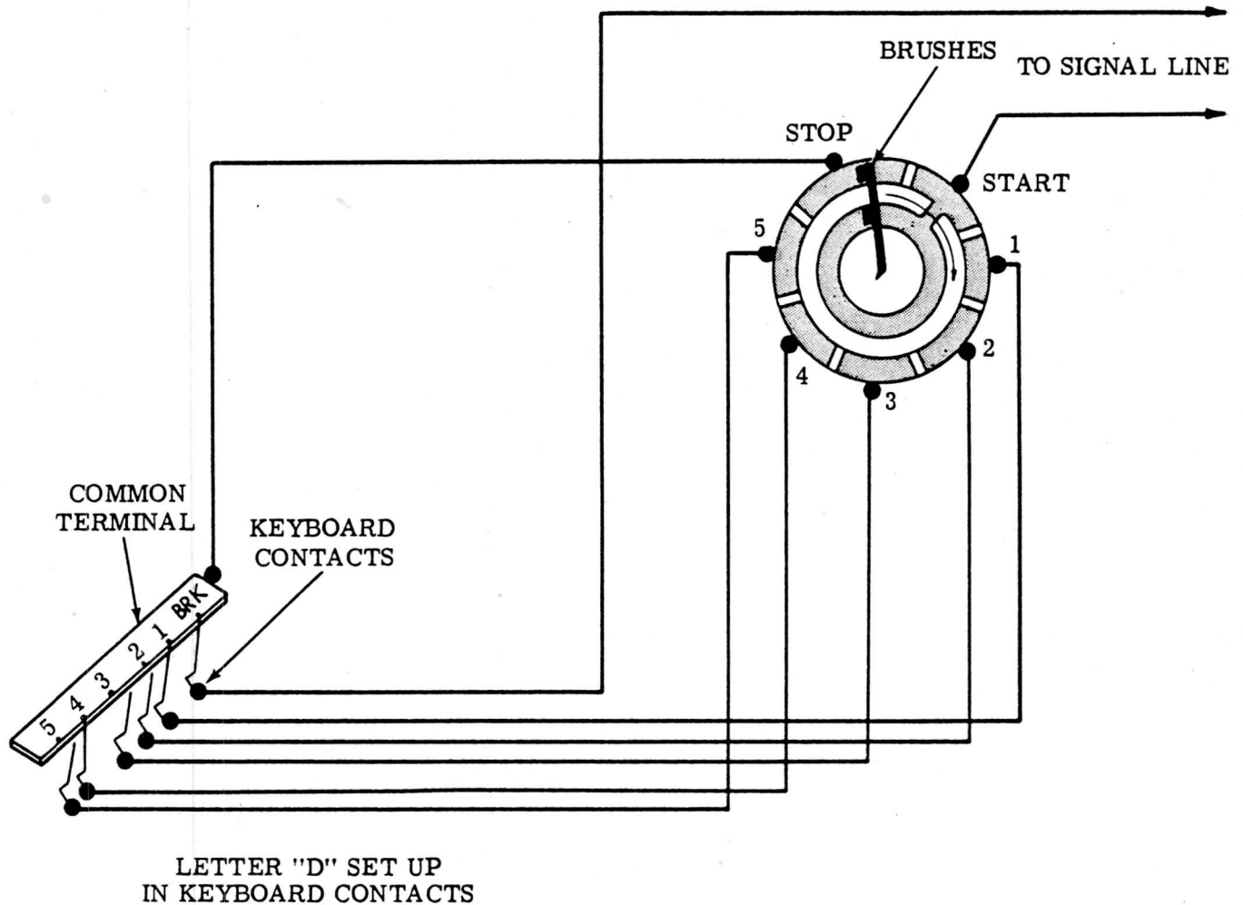
Figure 9 — Signal Wiring - 32 Typing Unit Distributor
