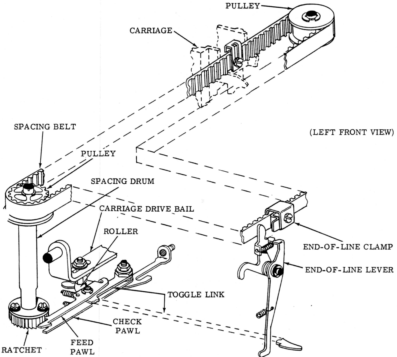
Figure 23 - Spacing Mechanism
