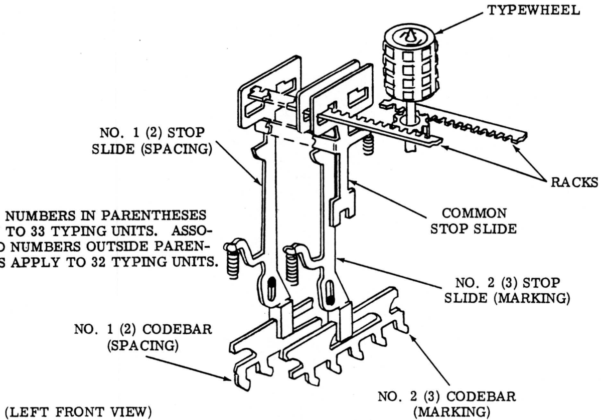
Figure 16 — Rotary Positioning Mechanism
