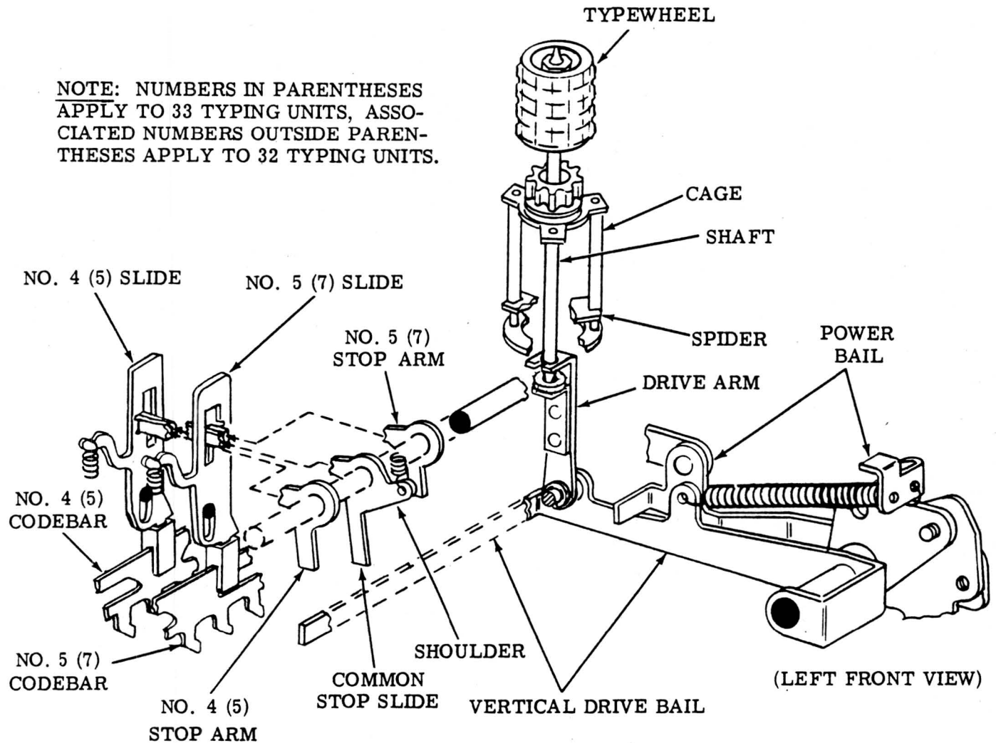
Figure 19 — Vertical Positioning Mechanism
