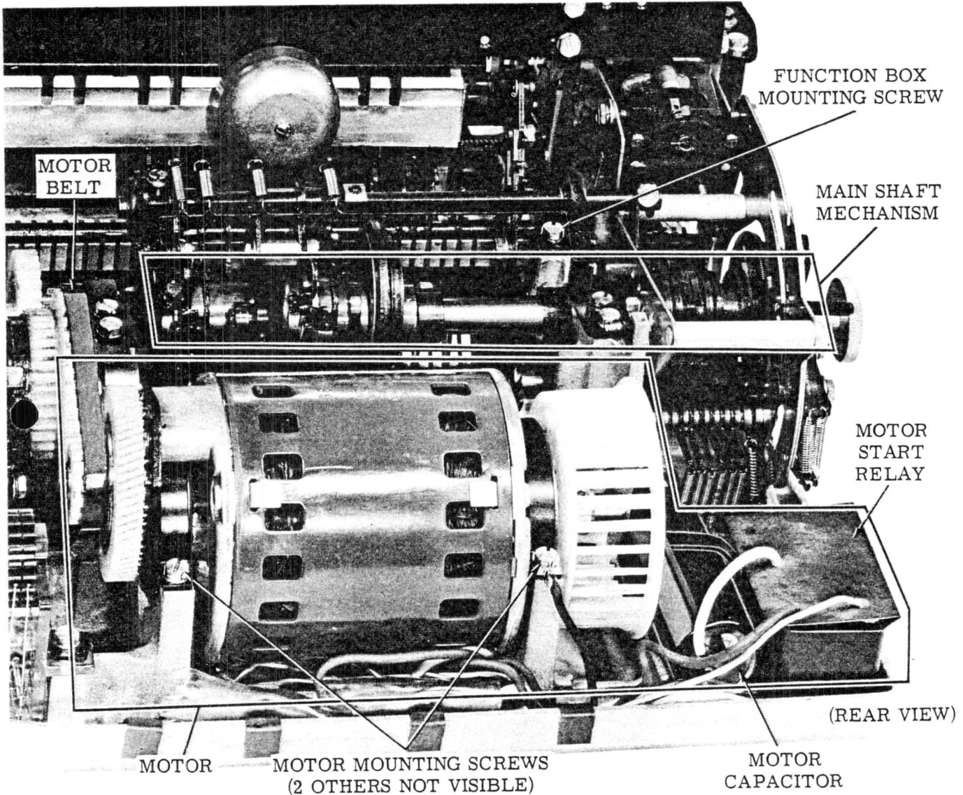
Figure 7 - Typing Unit
