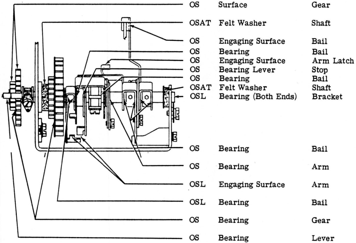
(TOP VIEW)
