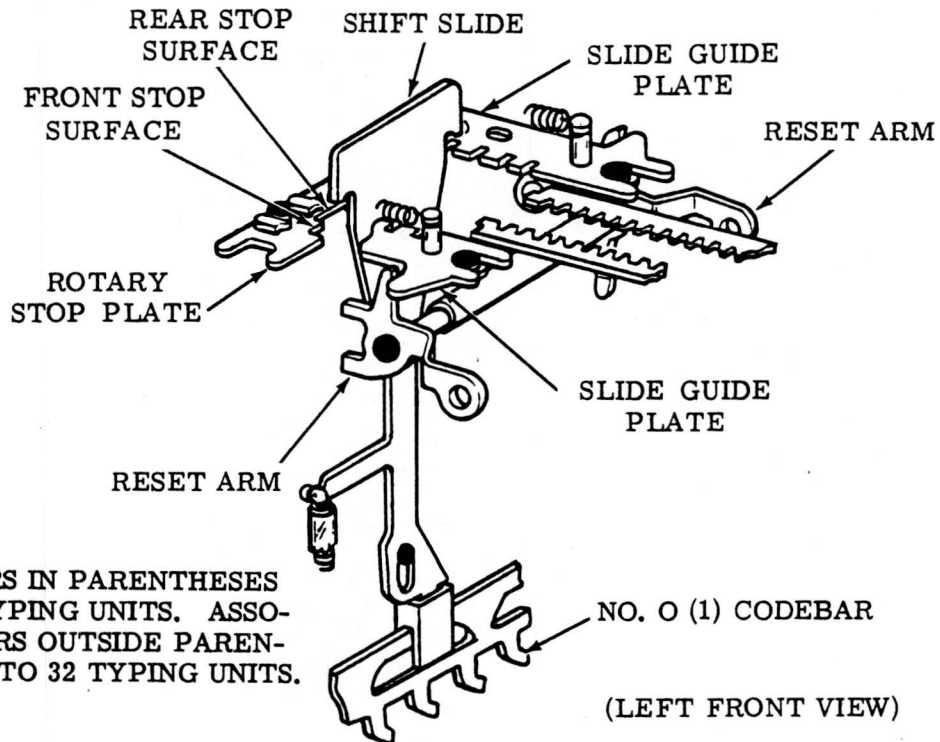
Figure 16 — Rotary Positioning Mechanism
