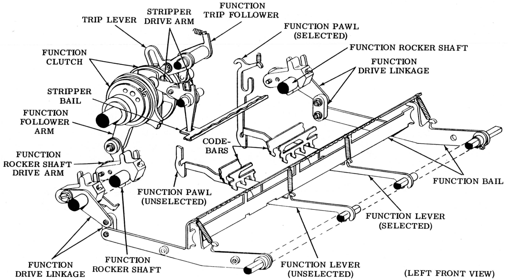
Figure 13 - Function Mechanism
