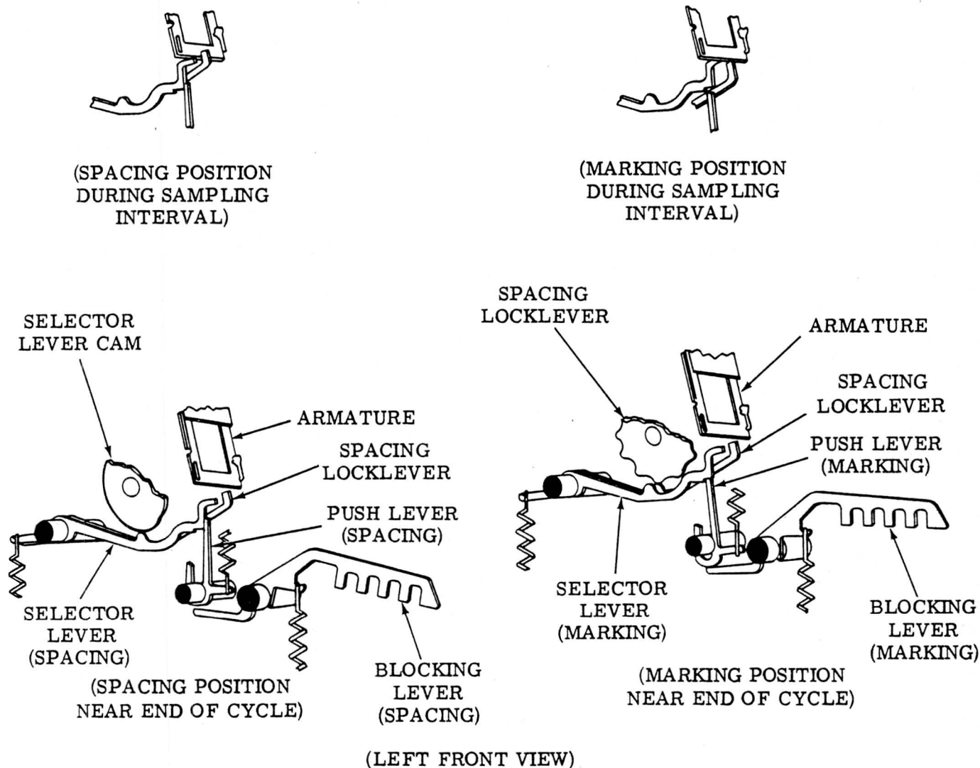
Figure 11 - Selector Mechanism
