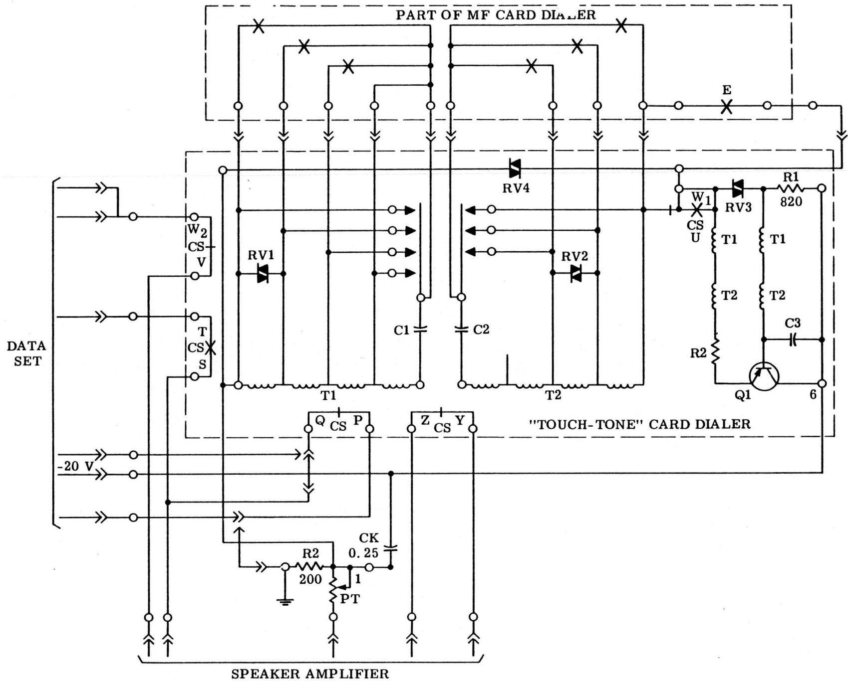
Figure 16 - TOUCH-TONE Card Dialer Circuit
