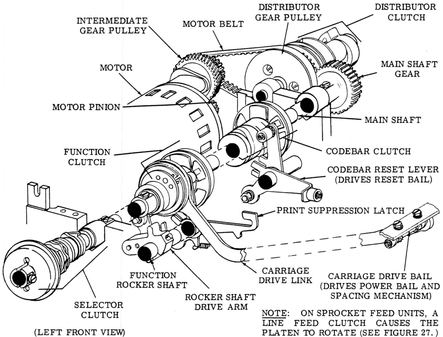
Figure 6 — Power Distribution
