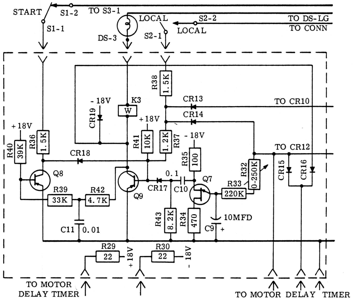
Figure 4 - Local Circuit
