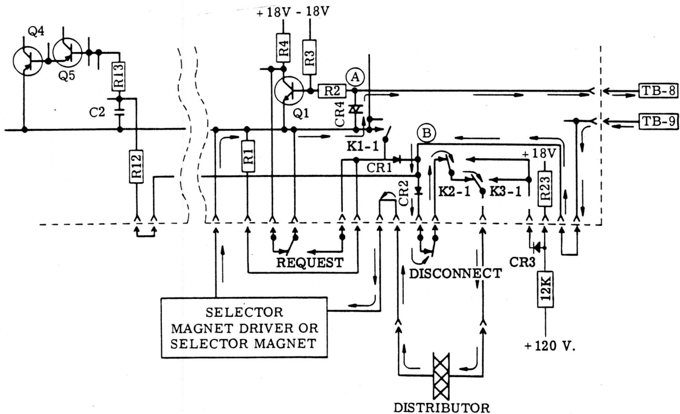
Figure 20 - Control Circuits in Connected Condition
