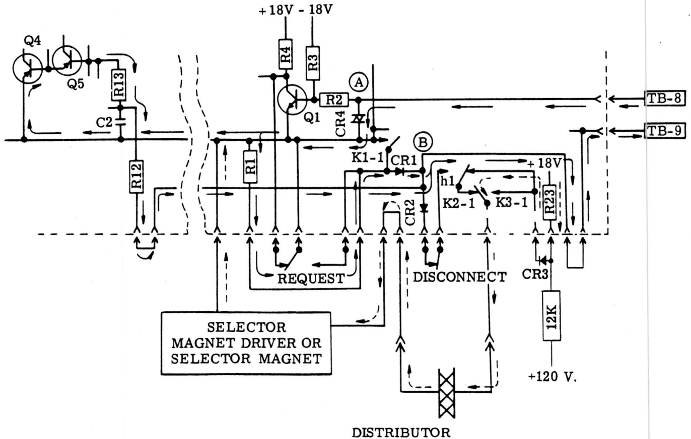
Figure 19 - Control Circuits in Idle Condition
