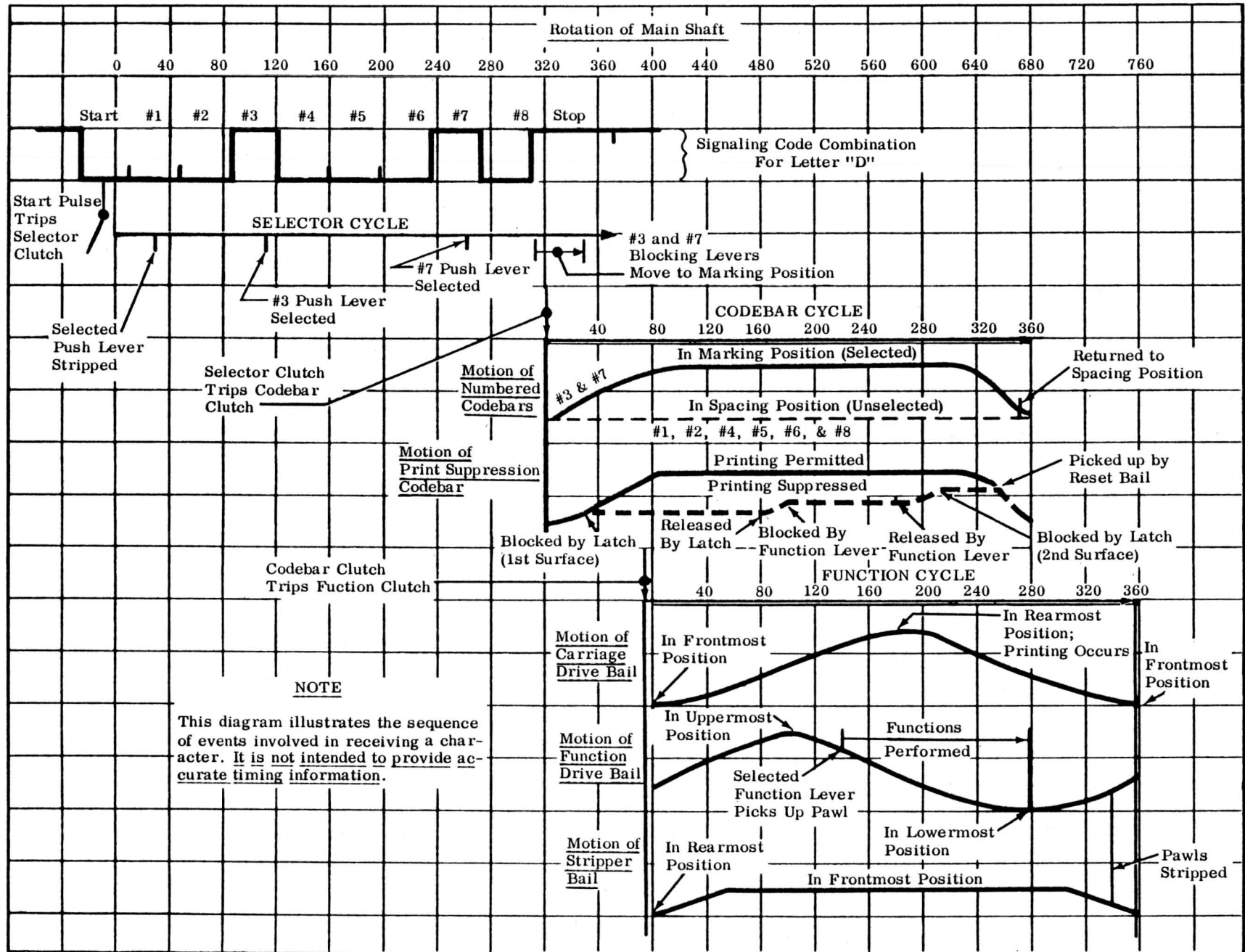
Figure 5 — Sequence Diagram - 33 Typing Unit Operation
