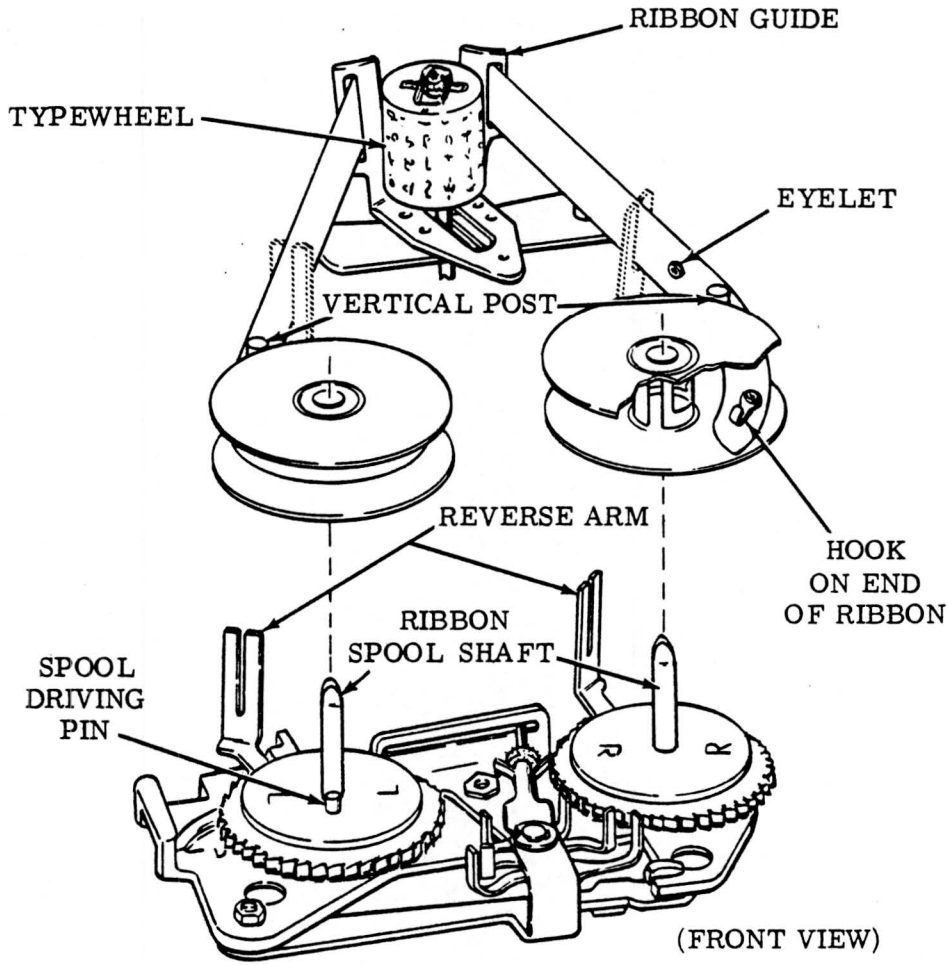
Figure 5 - Ribbon Threading
