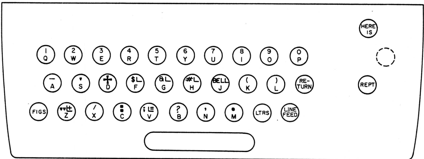
Figure 4 - 32 Keyboard Arrangement
