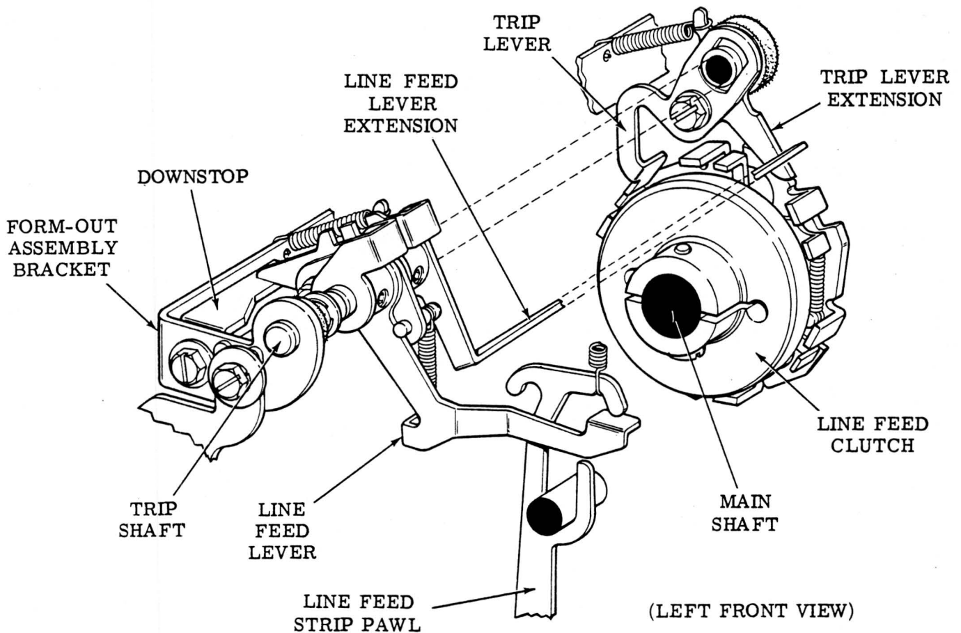
Figure 28 — Form-Out Mechanism (Sprocket Feed)
