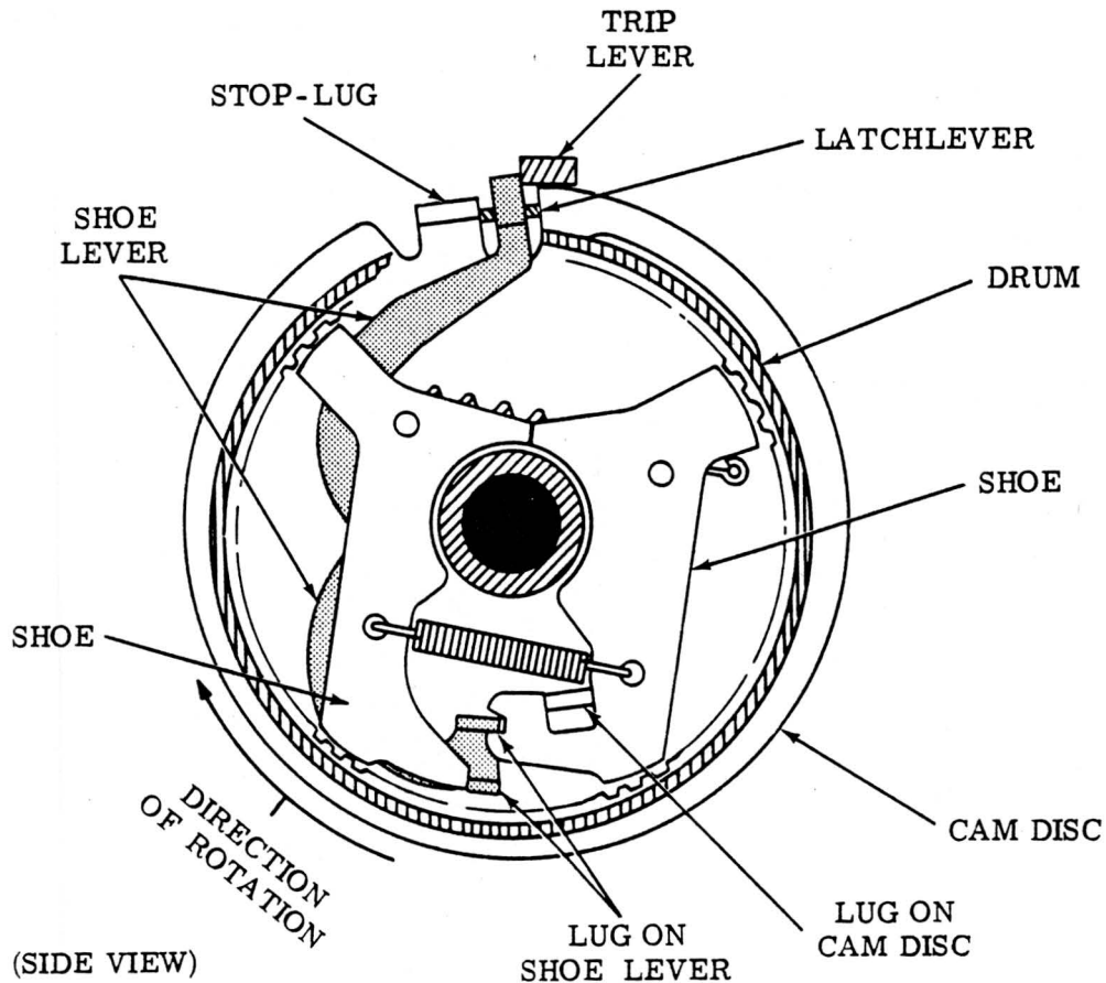
Figure 7 - Clutch
