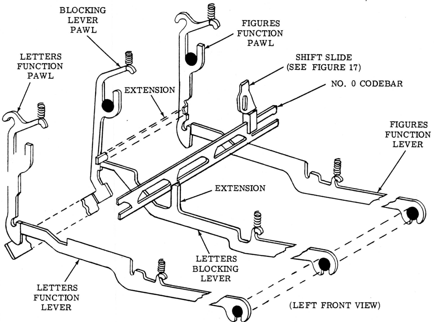
Figure 18 — Letters-Figures Shift Mechanism
