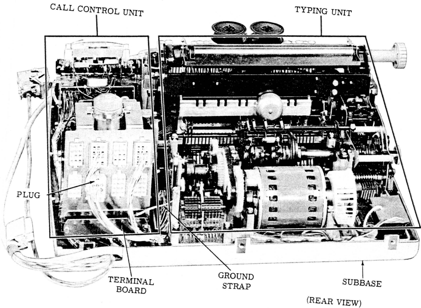
Figure 1 - Typing and Call Control Units
