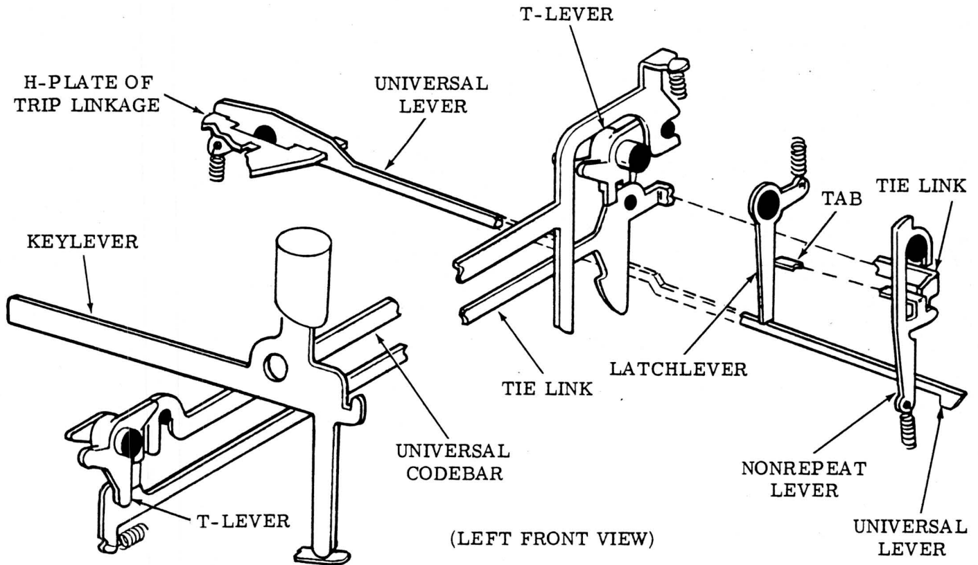
Figure 2 - Universal Codebar Mechanism
